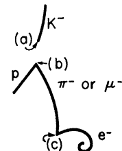
FIG. 1. A typical event satisfying the selection criteria. (a) K^- + \text{nucleus} \rightarrow \Lambda + \text{fragments} , (b) \Lambda \rightarrow p\pi^- or \Lambda \rightarrow p\mu^- \bar{\nu} , (c) \mu^- \rightarrow e^- \nu \bar{\nu} .
